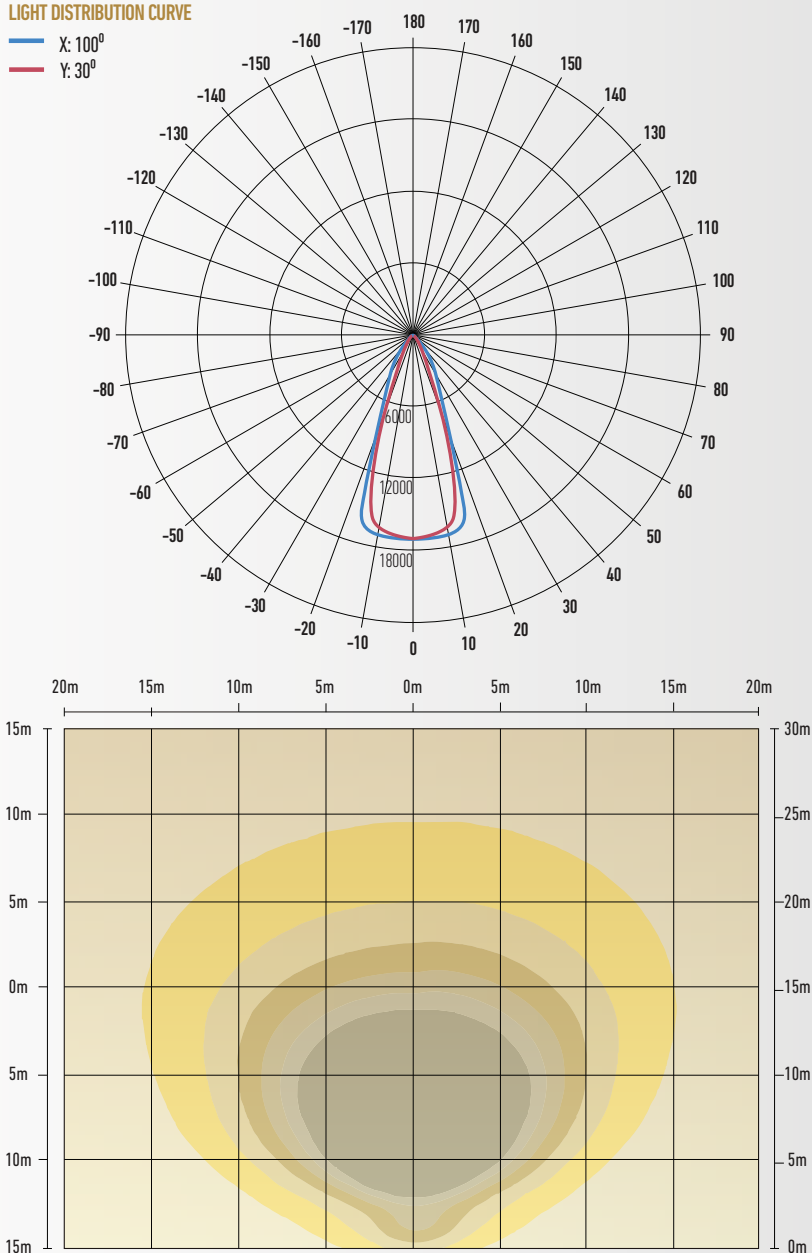
LIGHT DISTRIBUTION CURVE
